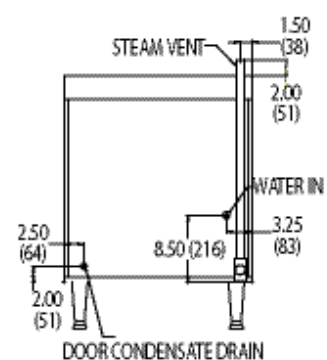
ALTAIR II - 4 PAN REAR VIEW
