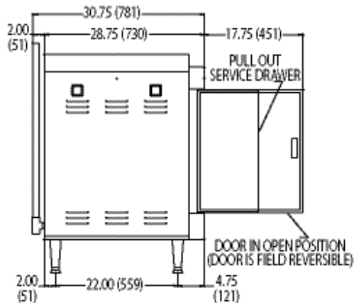
ALTAIR II - 6 PAN LEFT SIDE VIEW
