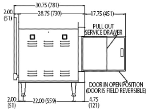
ALTAIR II - 4 PAN LEFT SIDE VIEW
