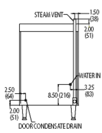
ALTAIR II - 6 PAN REAR VIEW
