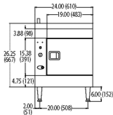
ALTAIR II - 4 PAN FRONT VIEW
