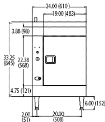
ALTAIR II - 6 PAN FRONT VIEW
